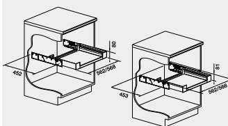
Flat Drawer 60 H
